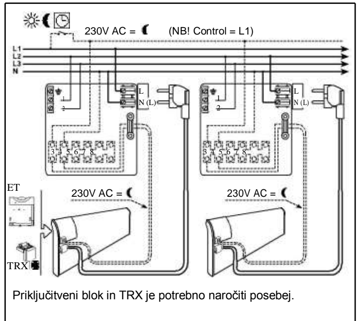
230 V diagram
